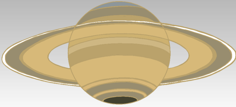
Saturn
